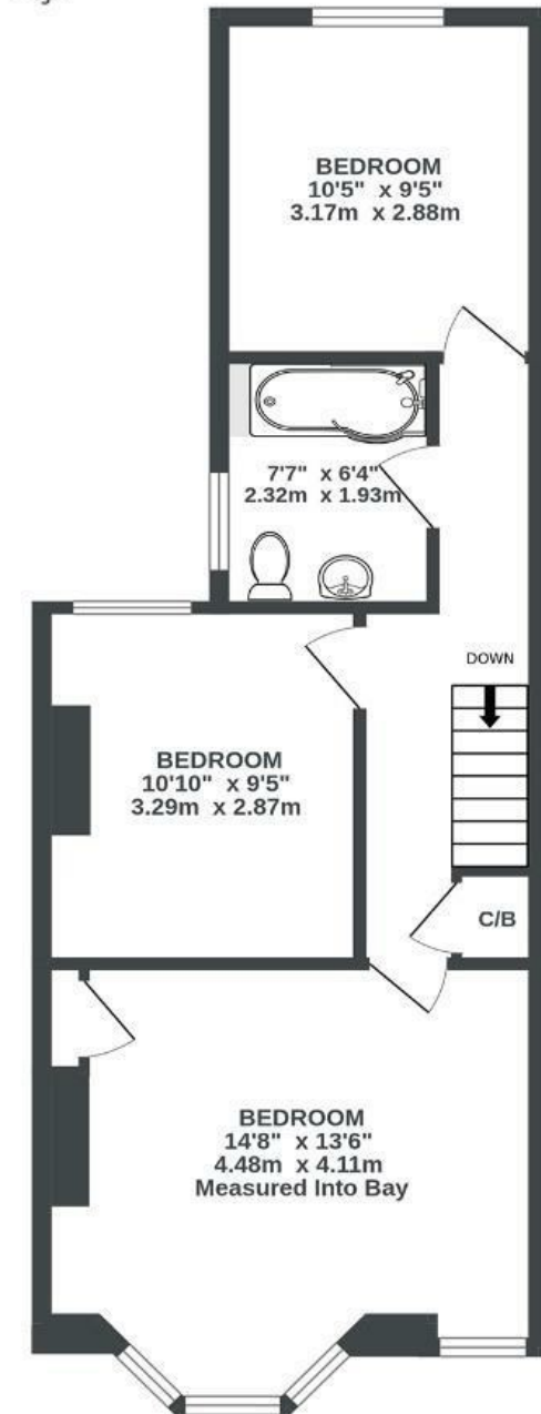
1ST FLOOR 499 sq.ft. (46.3 sq.m.) approx.
